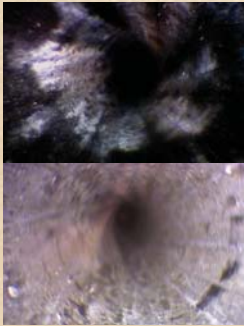
Bore scope photo of muzzleloader breech using a competitor's 209 primers after 2 shots.
